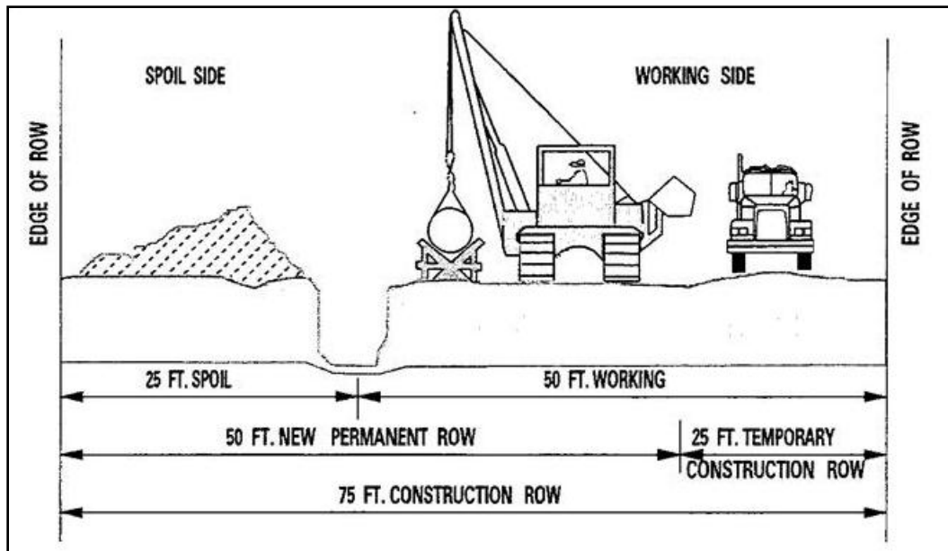
Figure 1. Typical 75-foot construction right-of-way.
